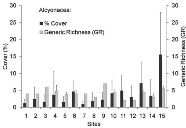
FIGURE 2. Percentage cover (%) and Generic Richness (GR) of Alcyonacea at each study site (mean values with standard deviations indicated where n>0).
